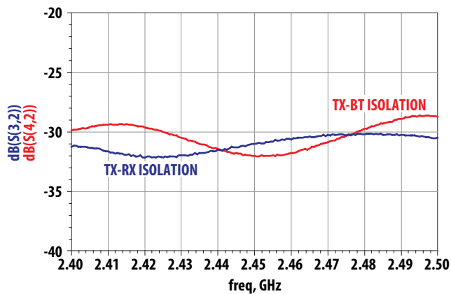
Figure 11. TX-RX and TX –BT Isolation in 2.4 – 2.5 GHz Band
